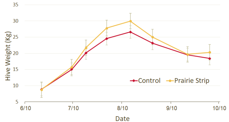
Fig. 2: Honey bee hives at farms with prairie strips were statistically heavier in 2017 and 2018 than hives without a strip (control). Data shown from 2018 ( p = 0.05 ).
